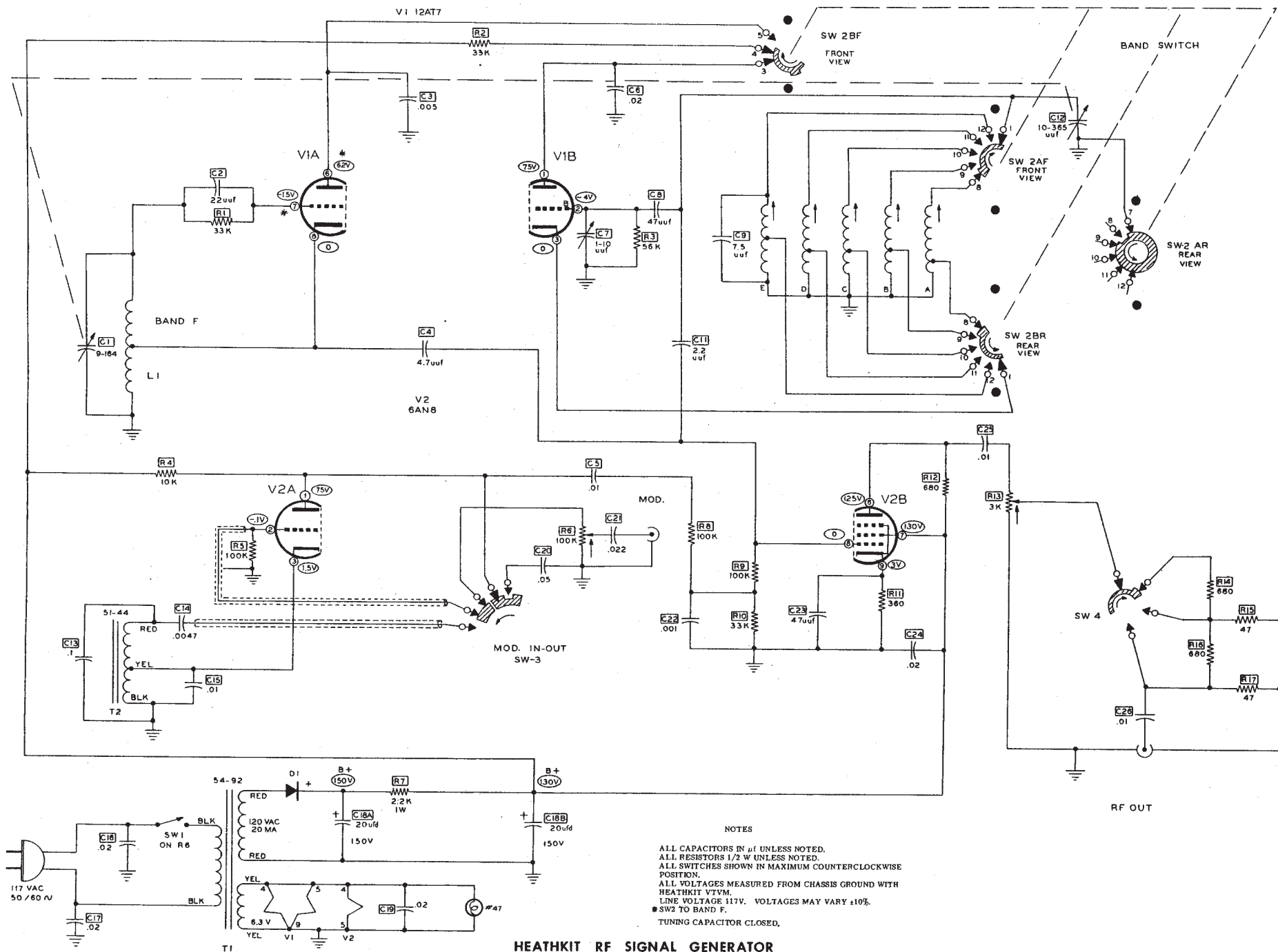
HEATHKIT RF SIGNAL GENERATOR MODEL RF-1
